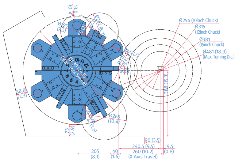
PUMA GT3100 (2axis, 12 option I )
