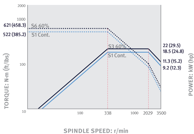
PUMA GT3100MA, PUMA GT3100LMA / DOOSAN FANUC i
