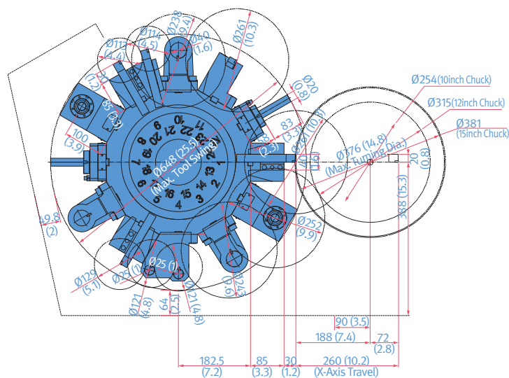
PUMA GT3100M (M, 24station, B option P )
