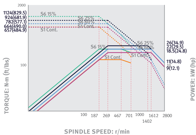
PUMA GT3100M, PUMA GT3100LM / DOOSAN FANUC i
