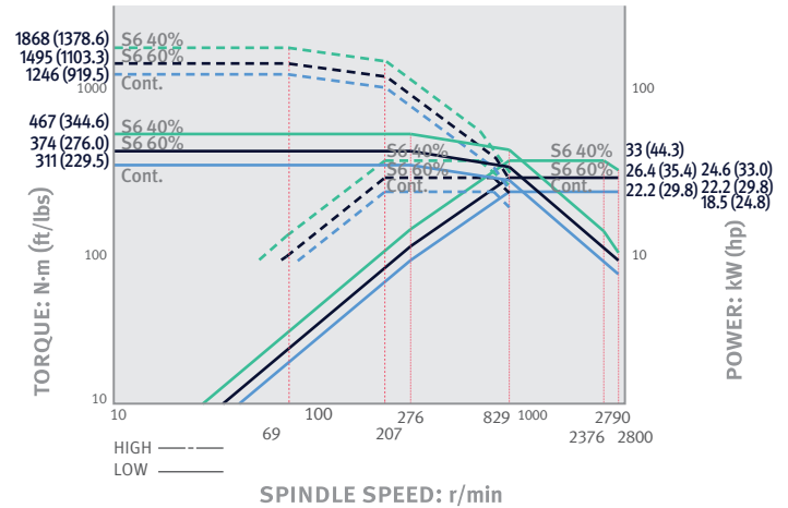
PUMA GT3100, PUMA GT3100L / SIEMENS S828D
