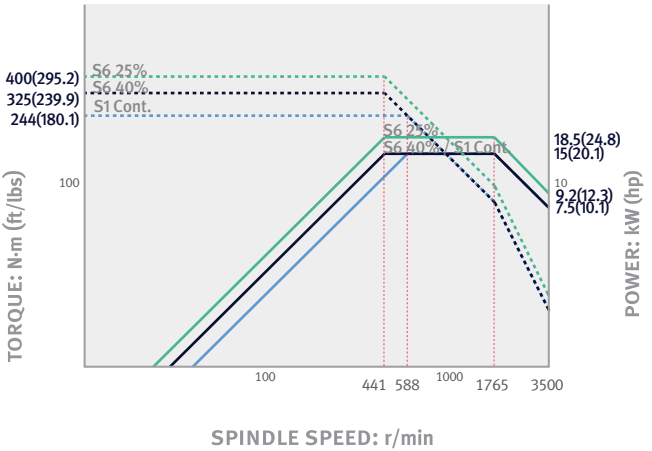
PUMA GT2100B, PUMA GT2100MB / DOOSAN FANUC i
