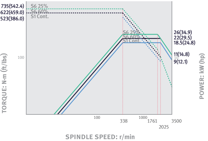
PUMA GT2600 series / DOOSAN FANUC i
