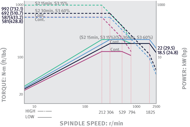
PUMA GT2600XLB / DOOSAN FANUC i
