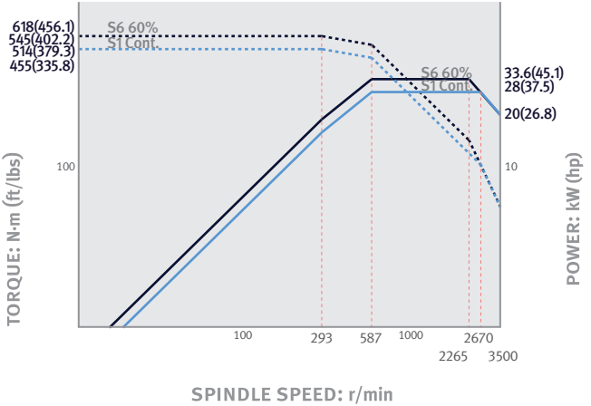
PUMA GT2600 series / SIEMENS S828D
