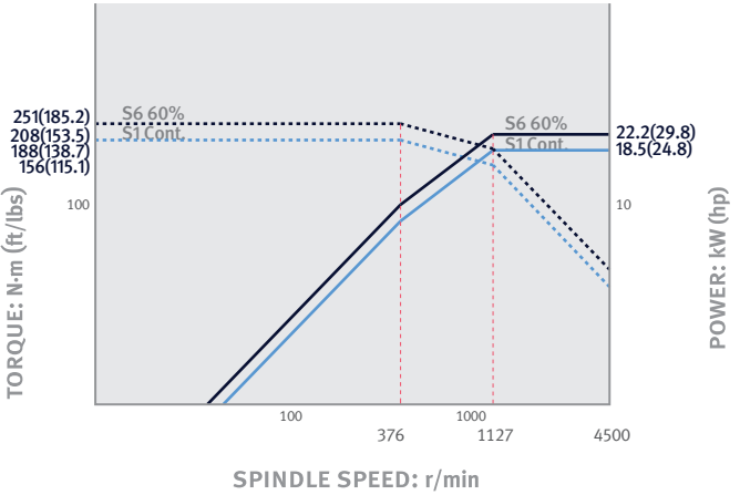
PUMA GT2100, PUMA GT2100M / SIEMENS S828D
