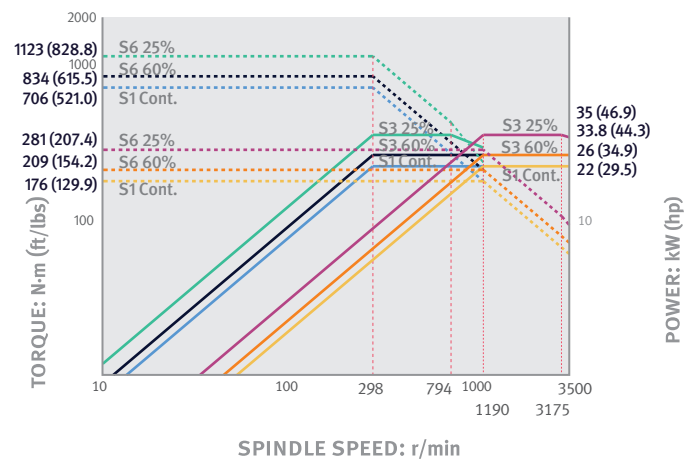
PUMA GT3100A, PUMA GT3100LA / DOOSAN FANUC i
